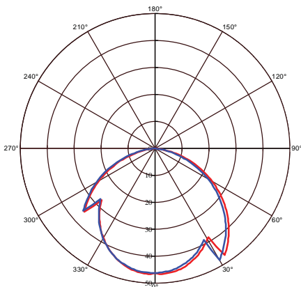
↳ C0 Plane beam angle(50%) ↳ C90 Plane beam angle(50%)
