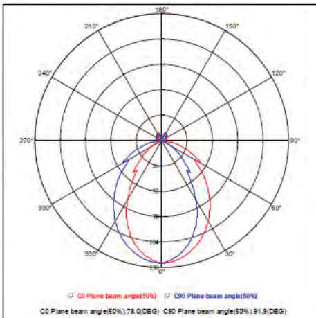
Photometric Diagram
