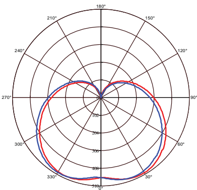
↳ C0 Plane beam angle(50%) ↳ C90 Plane beam angle(50%) C0 Plane beam angle(50%):200.2(DEG) C90 Plane beam angle(50%):199.8(DEG)
