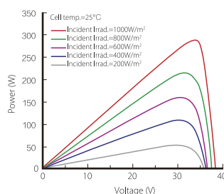
Power-Voltage Curve (LR6-60-290M)
