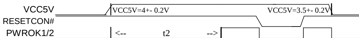
Figure 11-12. PWROK1/2 Timings
